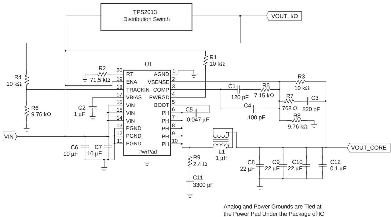
Figure 9. Application Circuit
