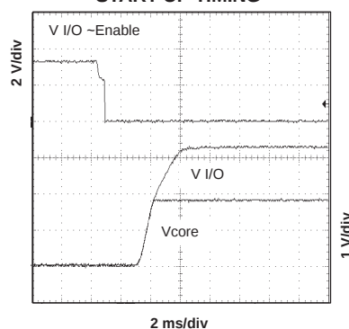
START-UP TIMING
