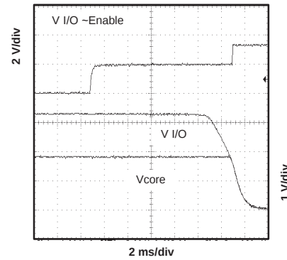
POWER-DOWN TIMING
